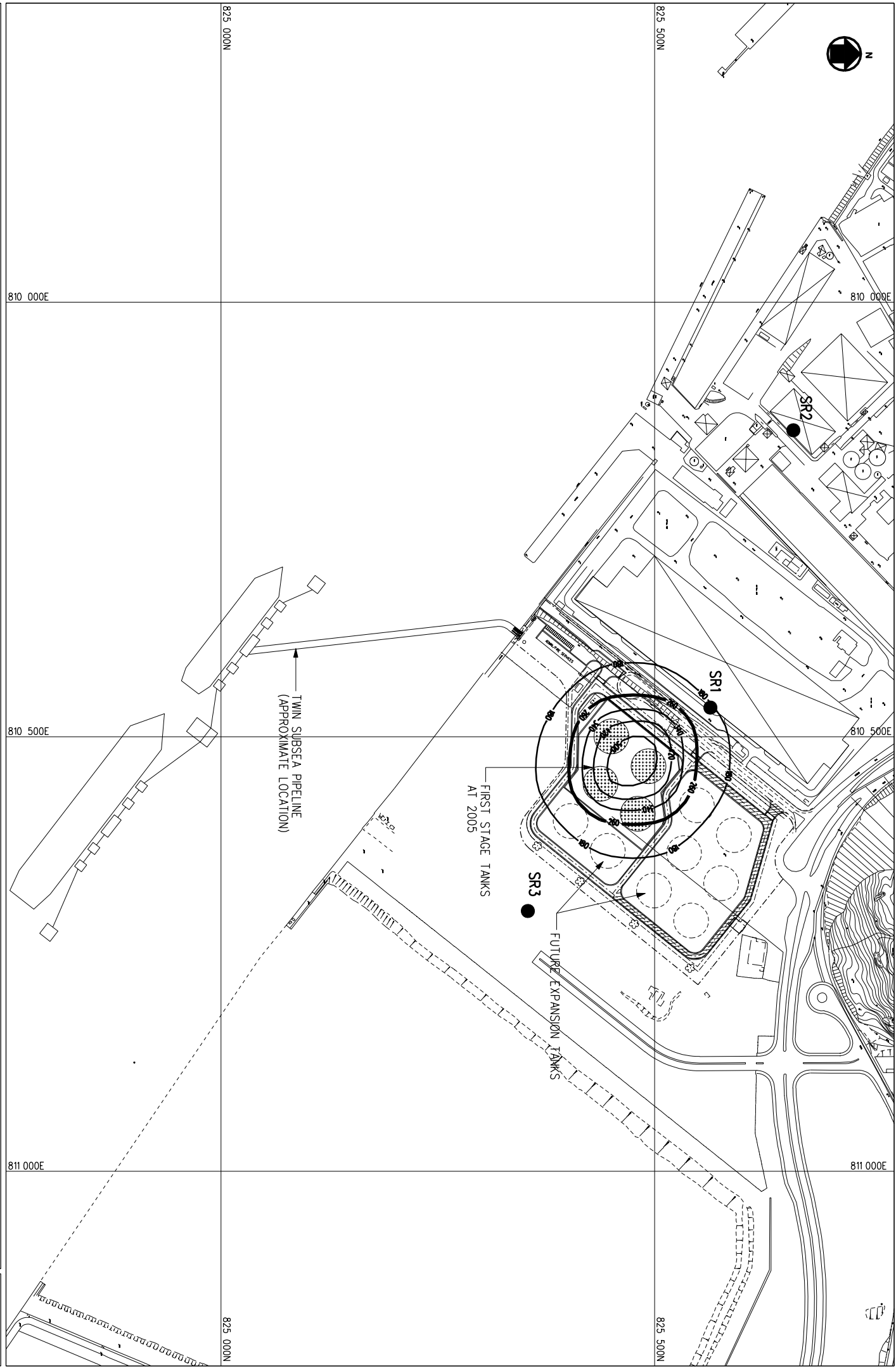
TSP (24-hours) Concentration (ug/m 3 ) Contours During Construction
